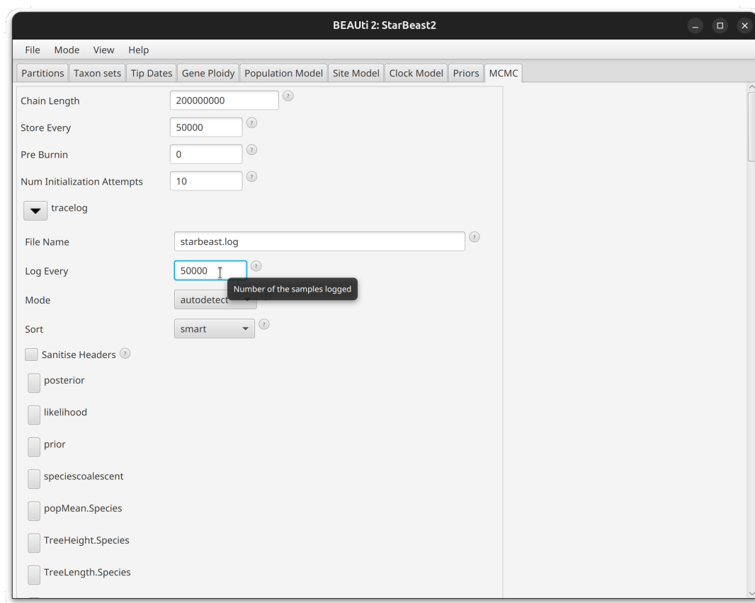
Figure 26: Changing the sampling rates after setting a chain length of 200 million
