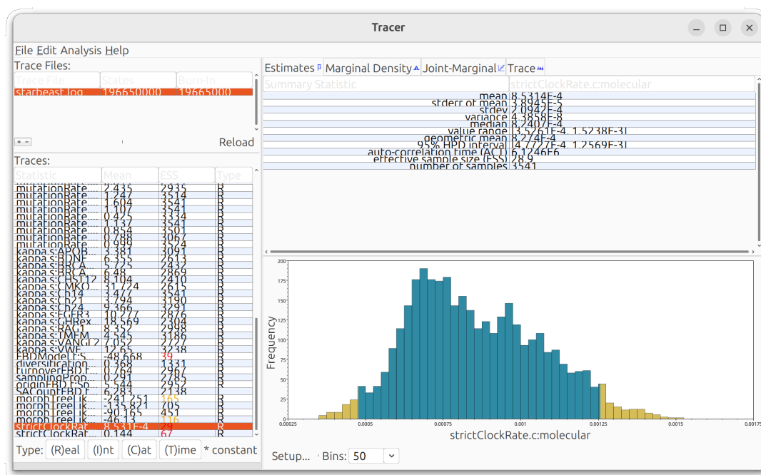
Figure 27: The estimated posterior distribution of the molecular clock rate
