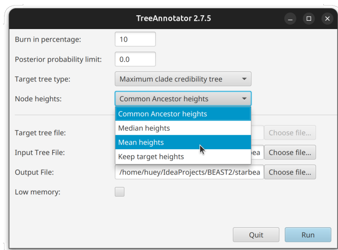
Figure 30: Running Tree Annotator for sampled ancestor trees
