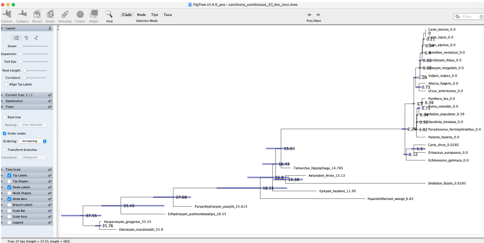
Figure 14: Summarised MCC tree of logged trees under the Brownian motion model.
