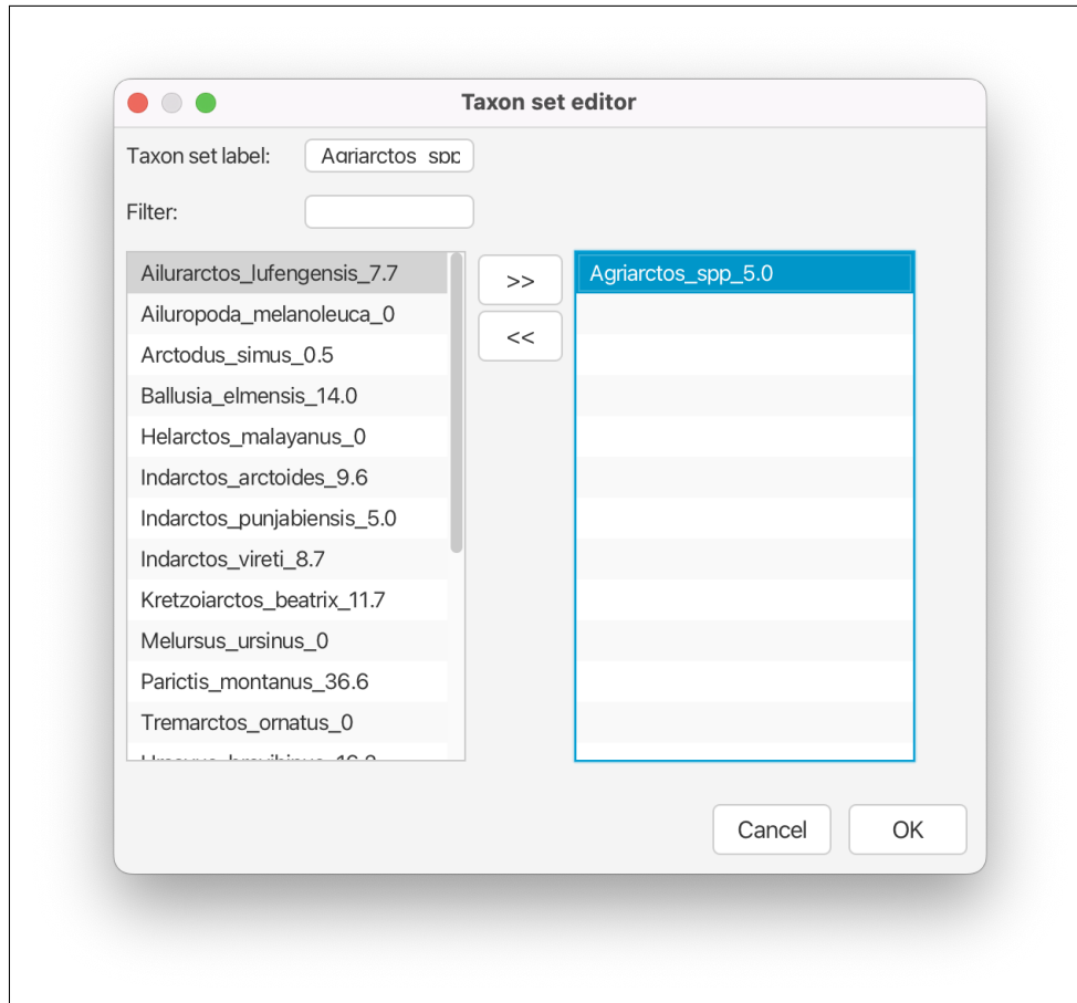
Figure 26: The Taxon set editor used to create the clade containing the Agriarctos spp. fossil.
