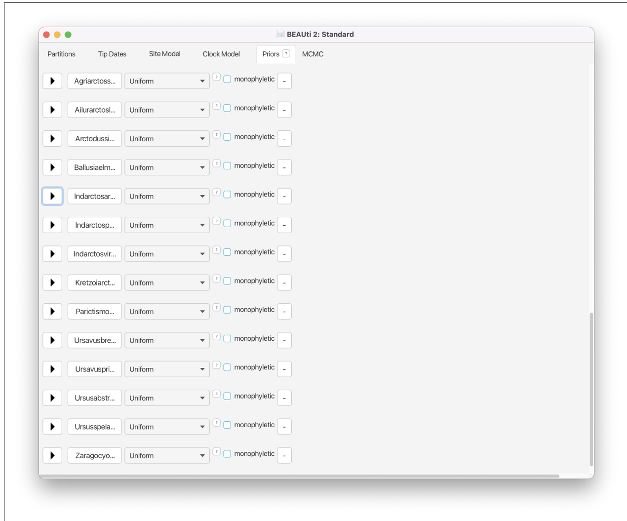
Figure 28: The Priors window showing the prior set on the ages of all fossils.
