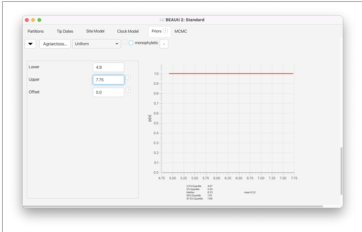
Figure 27: The Priors window showing the prior set on the age of the Agriarctos spp. fossil.
