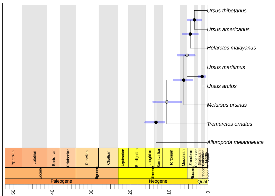
Figure 32: The maximum clade credibility tree of extant bears summarized by TreeAnnotator and plotted against stratigraphy using the strap package in R (see how to do this in Section 3.4.5 below). The internal nodes of the tree are indicated with circles, where circles mark nodes with posterior probability: \bullet \geq 0.95 , 0.95 > \bullet \geq 0.75 , 0.75 > \bullet . The 95% credible intervals for node ages are shown with transparent blue bars.
